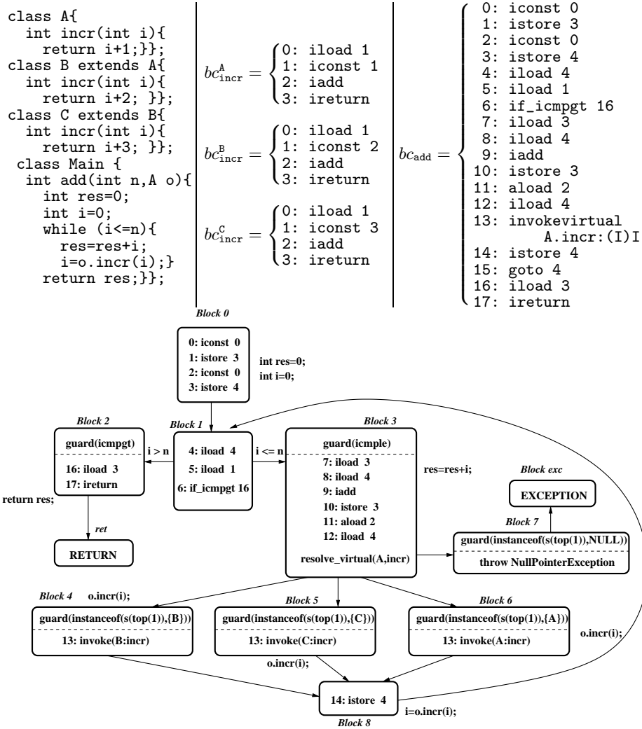
Fig. 1. The running example in source code, bytecode, and control flow graph
